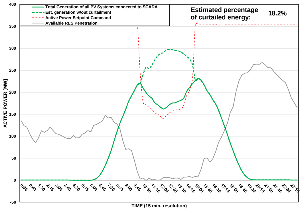
Scada PVs Generation on 04/08/2025 (curtailment time: 10:00 - 14:45)
