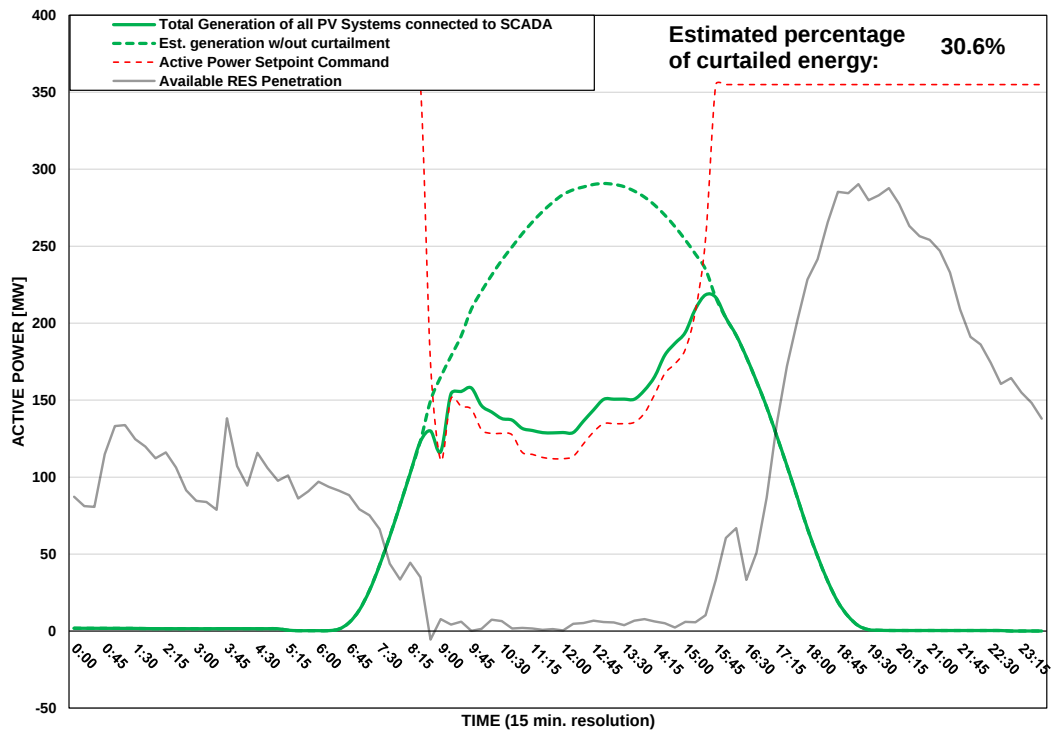
Scada PVs Generation on 23/08/2025 (curtailment time: 08:45 - 15:30)
