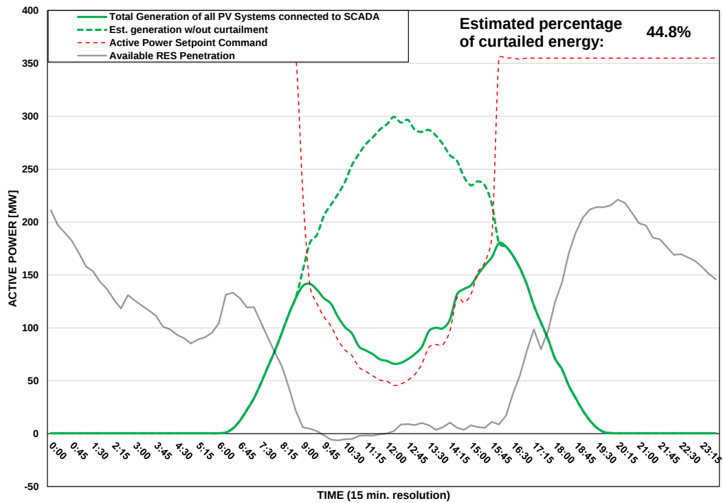
Scada PVs Generation on 02/08/2025 (curtailment time: 09:00 - 15:45)
