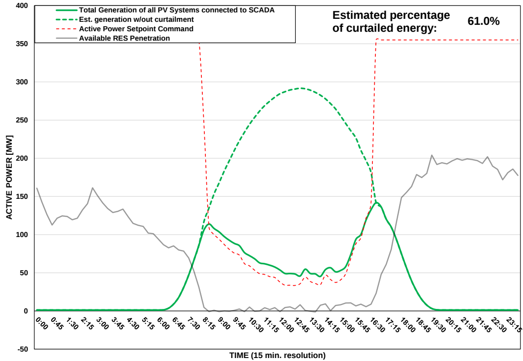
Scada PVs Generation on 15/08/2025 (curtailment time: 08:15 - 16:30)
