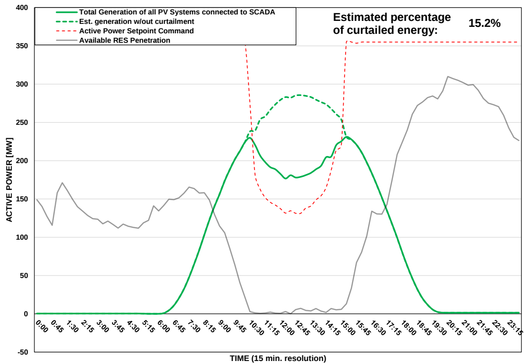
Scada PVs Generation on 05/08/2025 (curtailment time: 10:30 - 15:00)
