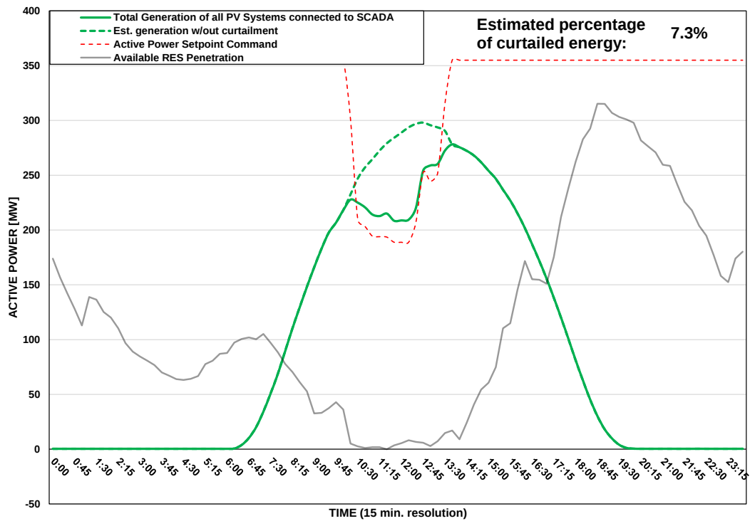
Scada PVs Generation on 08/08/2025 (curtailment time: 10:15 - 13:30)
