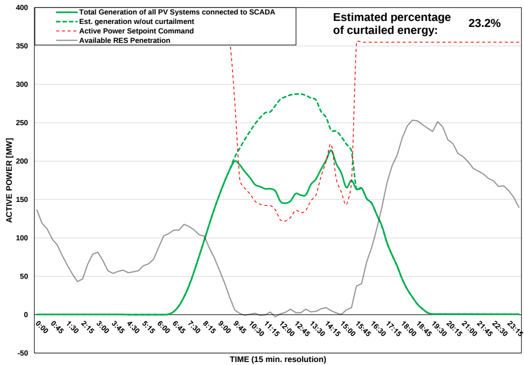
Scada PVs Generation on 27/08/2025 (curtailment time: 09:45 - 15:30)
