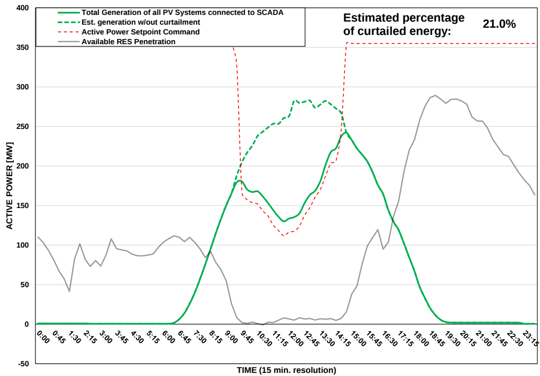
Scada PVs Generation on 21/08/2025 (curtailment time: 09:30 - 14:30)
