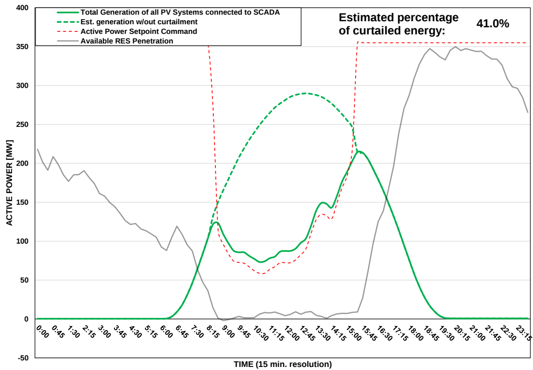
Scada PVs Generation on 10/08/2025 (curtailment time: 08:30 - 15:15)
