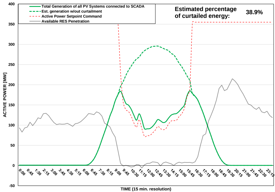
Scada PVs Generation on 18/08/2025 (curtailment time: 09:30 - 16:00)
