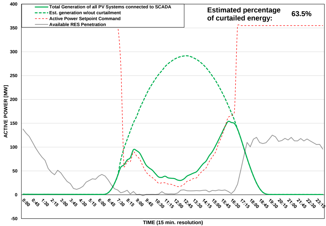
Scada PVs Generation on 31/08/2025 (curtailment time: 07:45 - 16:45)
