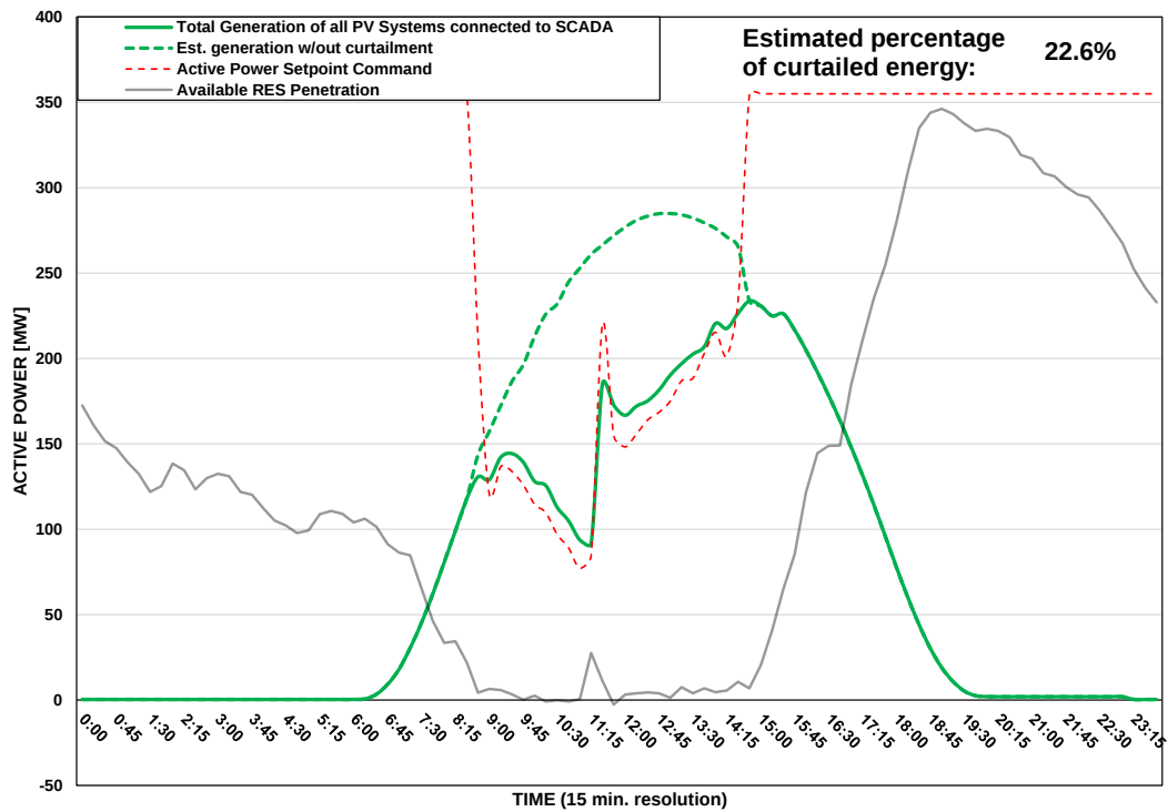
Scada PVs Generation on 09/08/2025 (curtailment time: 08:45 - 14:30)
