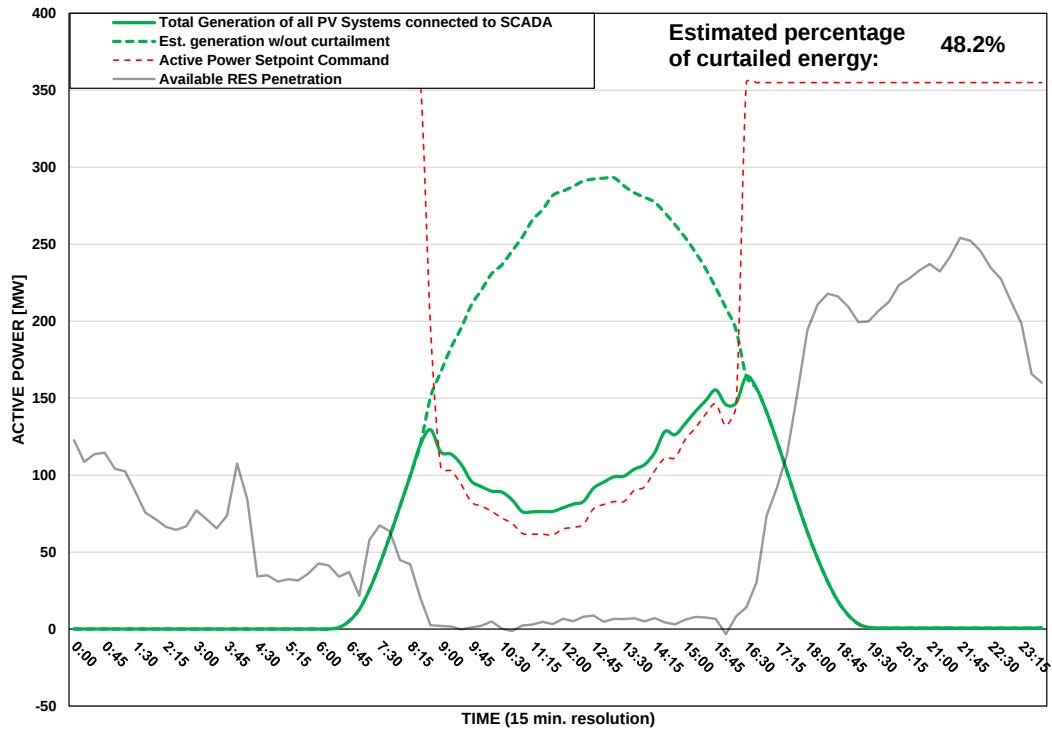
Scada PVs Generation on 24/08/2025 (curtailment time: 08:45 - 16:15)
