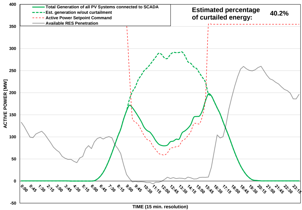
Scada PVs Generation on 01/08/2025 (curtailment time: 09:15 - 15:45)
