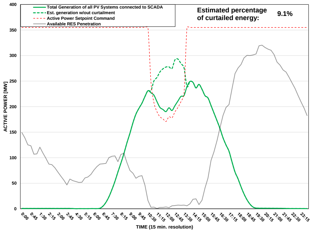
Scada PVs Generation on 25/08/2025 (curtailment time: 10:45 - 13:30)
