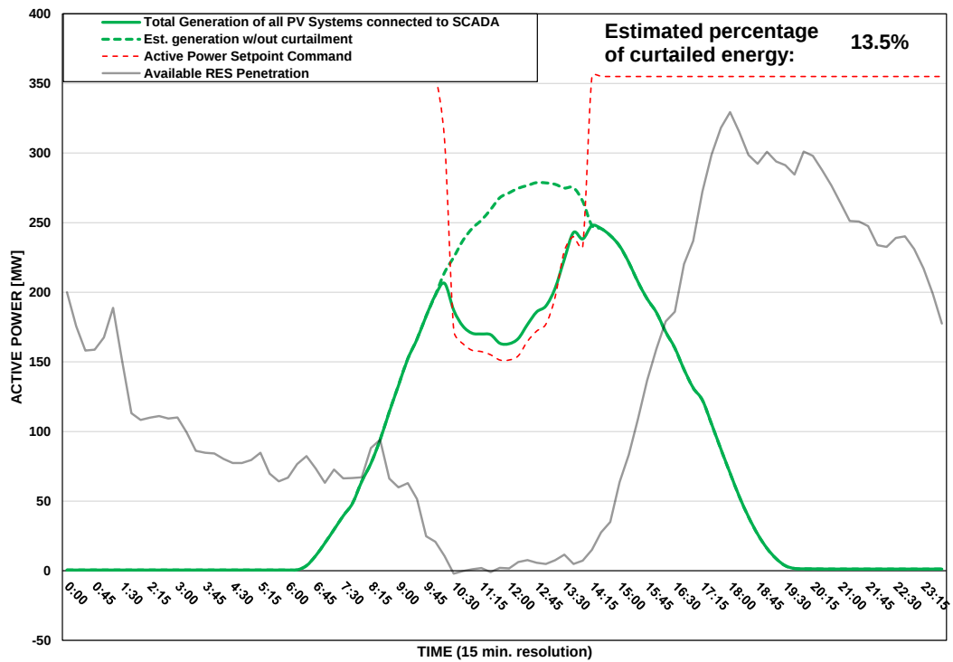
Scada PVs Generation on 14/08/2025 (curtailment time: 10:15 - 14:00)
