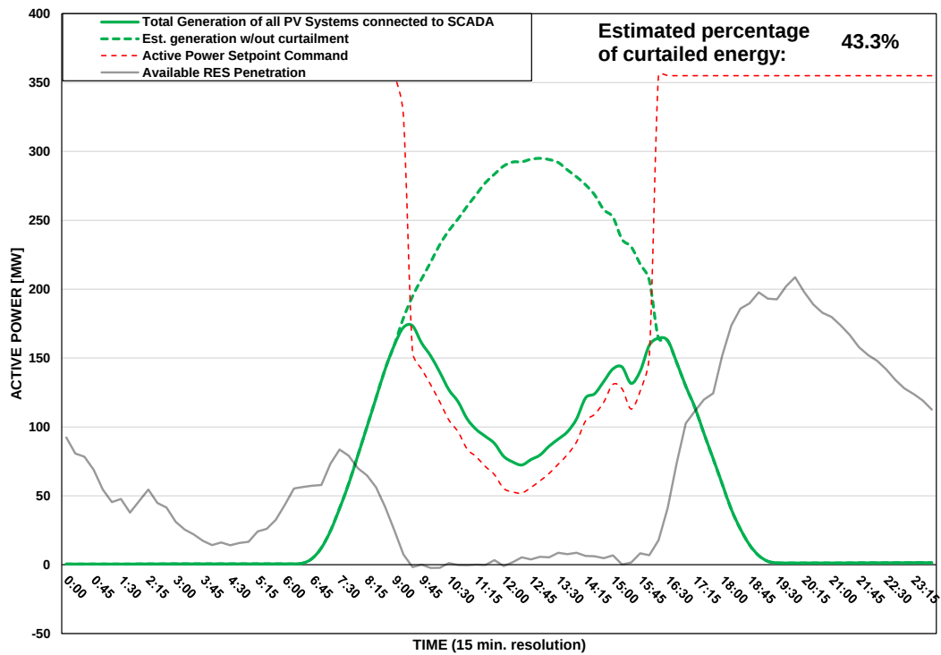
Scada PVs Generation on 29/08/2025 (curtailment time: 09:15 - 16:00)
