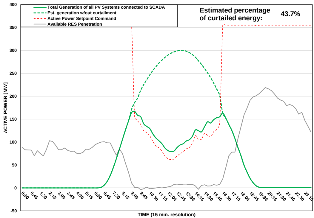
Scada PVs Generation on 20/08/2025 (curtailment time: 09:00 - 16:15)
