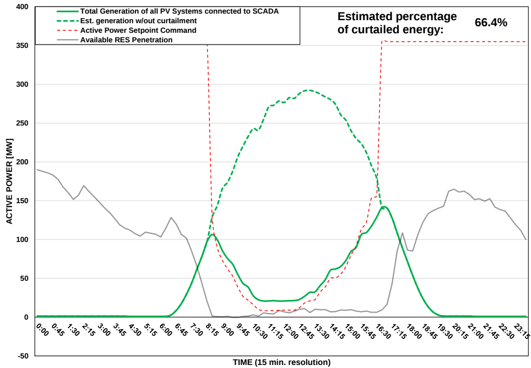
Scada PVs Generation on 17/08/2025 (curtailment time: 08:30 - 16:30)
