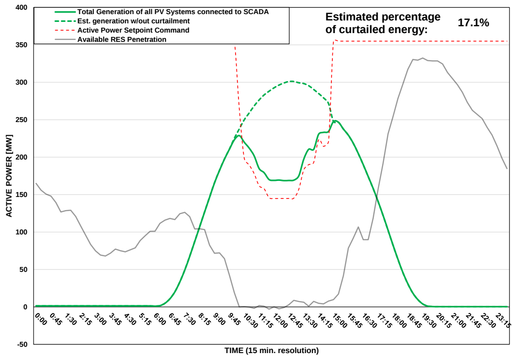
Scada PVs Generation on 07/08/2025 (curtailment time: 10:00 - 14:45)
