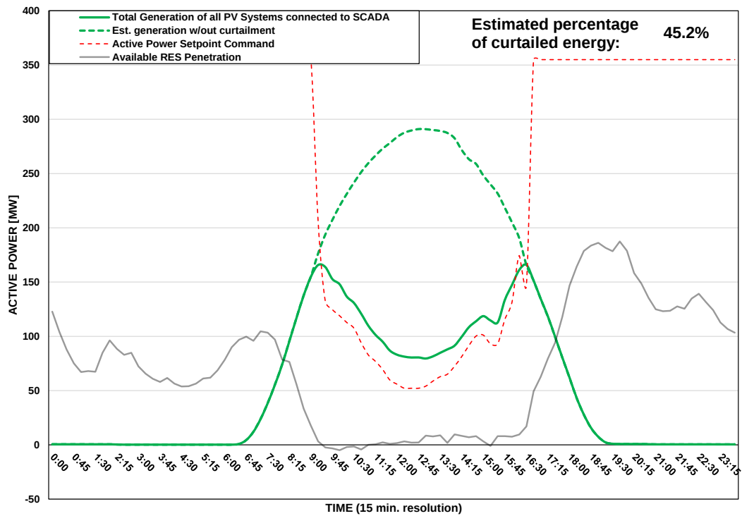
Scada PVs Generation on 28/08/2025 (curtailment time: 09:15 - 16:15)
