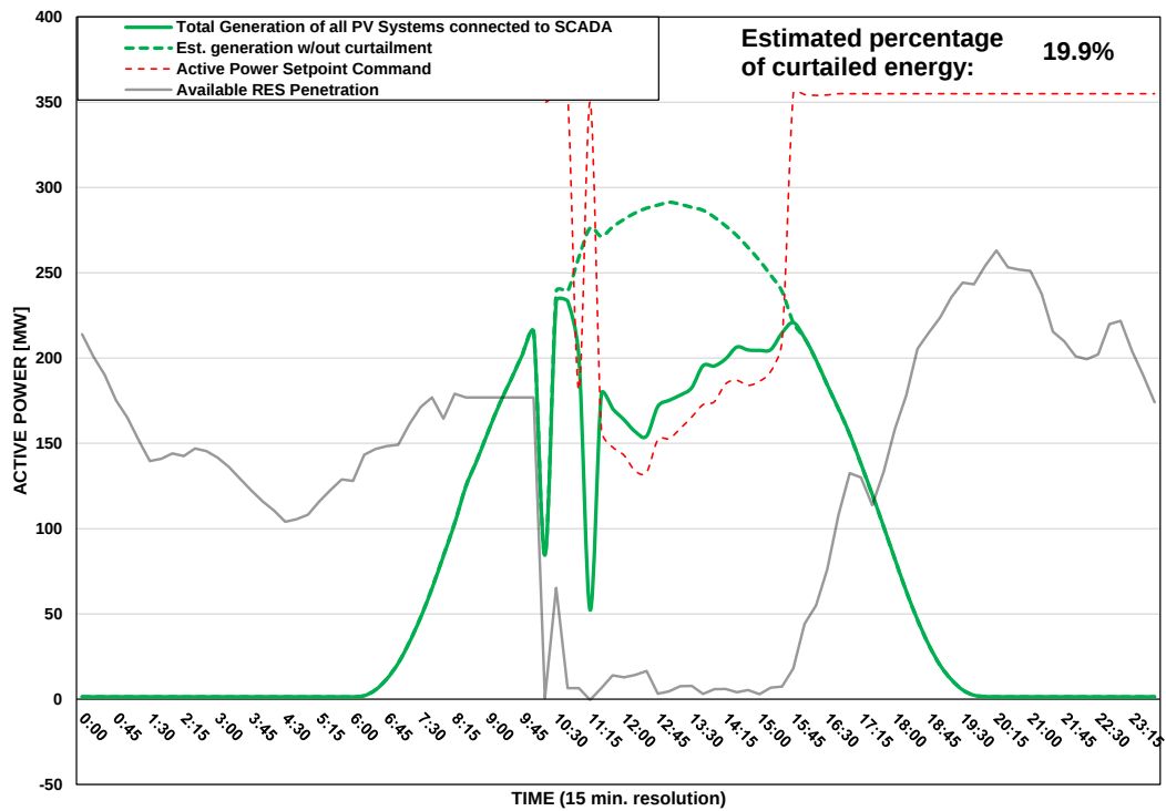
Scada PVs Generation on 06/08/2025 (curtailment time: 10:30 - 15:30)
