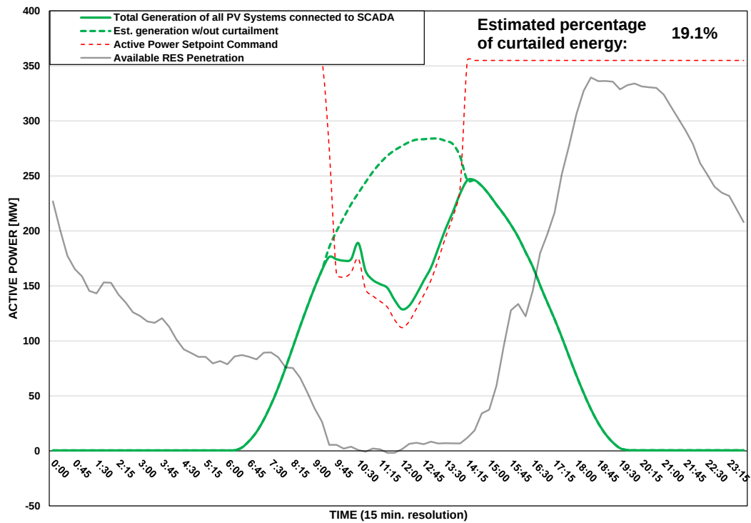
Scada PVs Generation on 13/08/2025 (curtailment time: 09:30 - 14:00)
