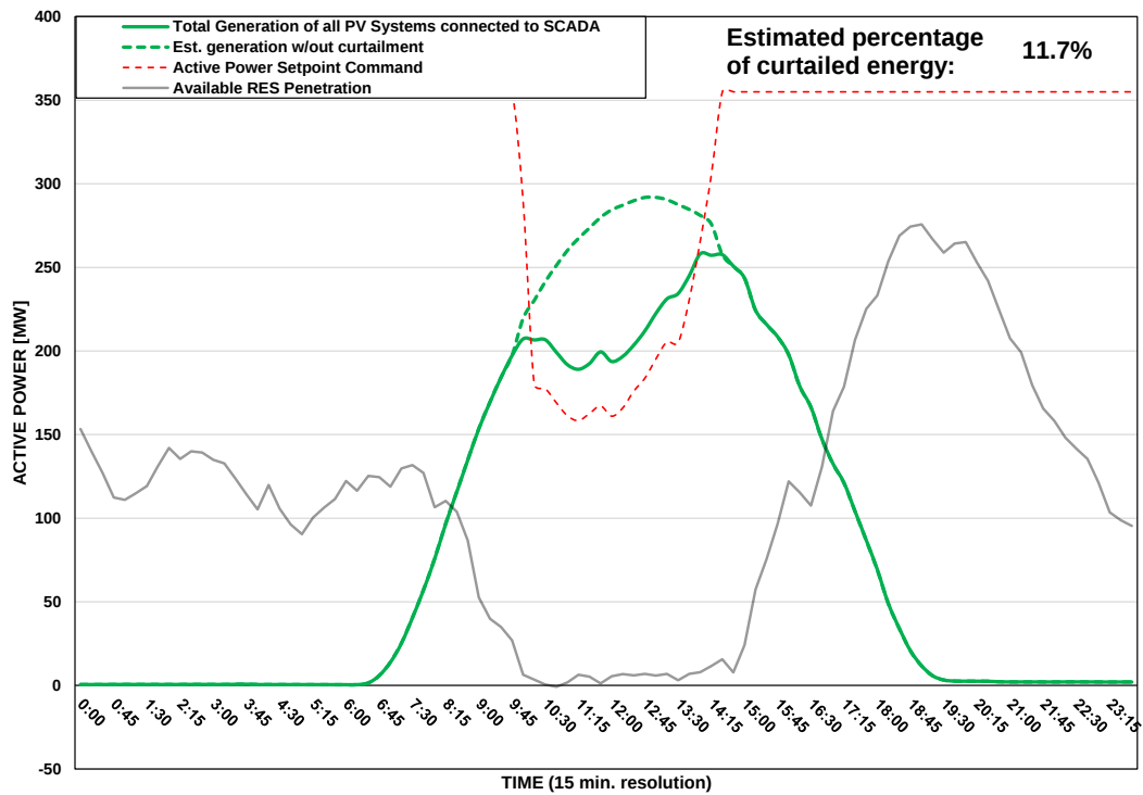
Scada PVs Generation on 22/08/2025 (curtailment time: 10:00 - 14:15)
