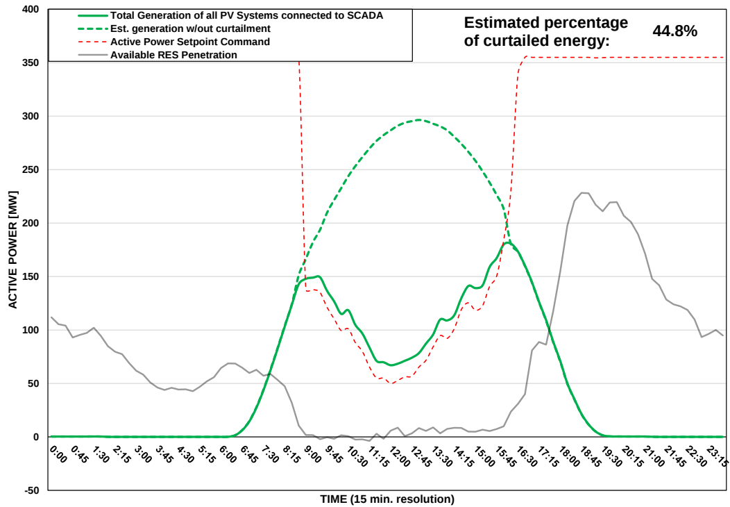
Scada PVs Generation on 19/08/2025 (curtailment time: 08:45 - 16:00)
