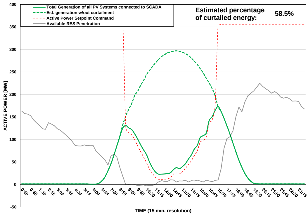
Scada PVs Generation on 16/08/2025 (curtailment time: 08:30 - 16:15)
