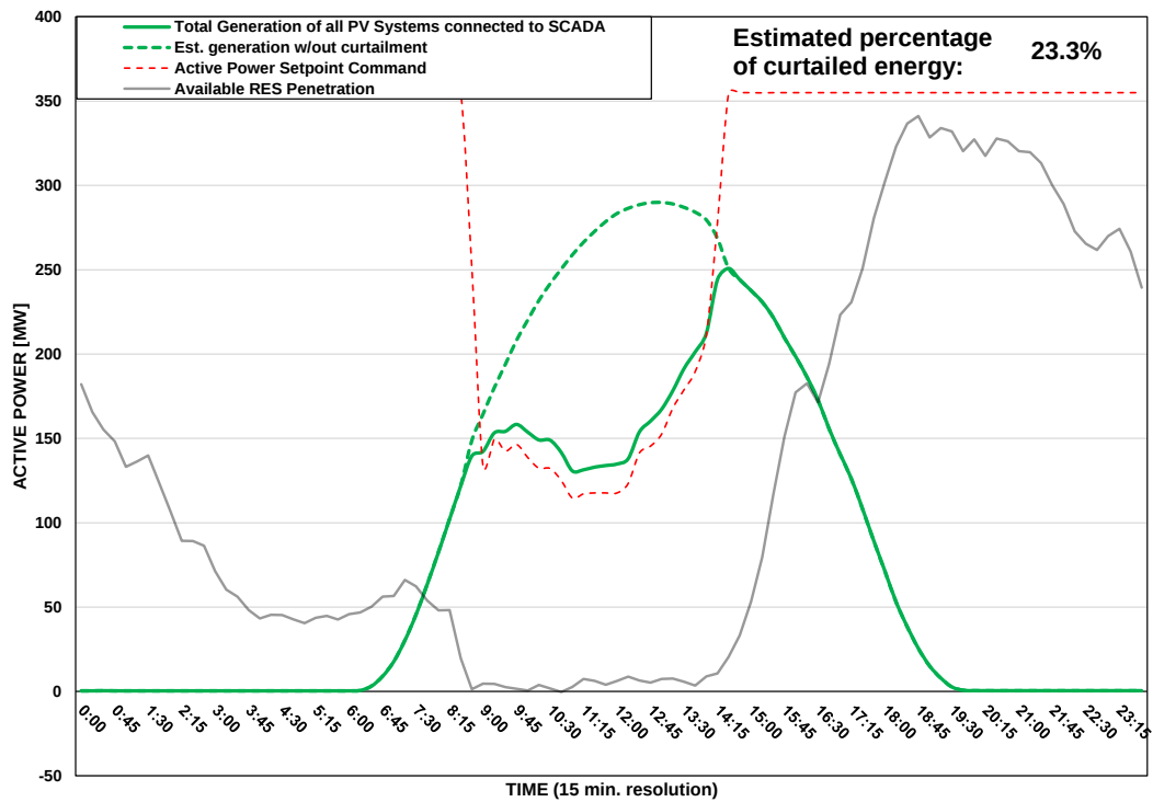
Scada PVs Generation on 12/08/2025 (curtailment time: 08:45 - 14:15)
