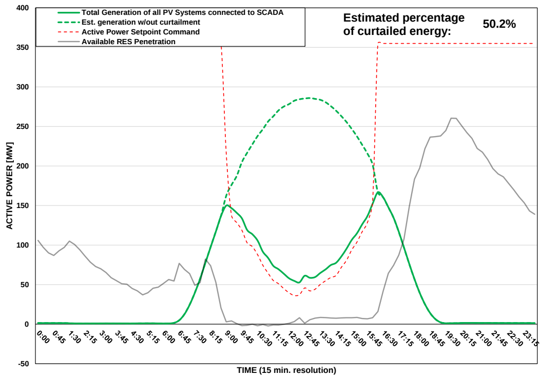
Scada PVs Generation on 30/08/2025 (curtailment time: 09:00 - 16:00)
