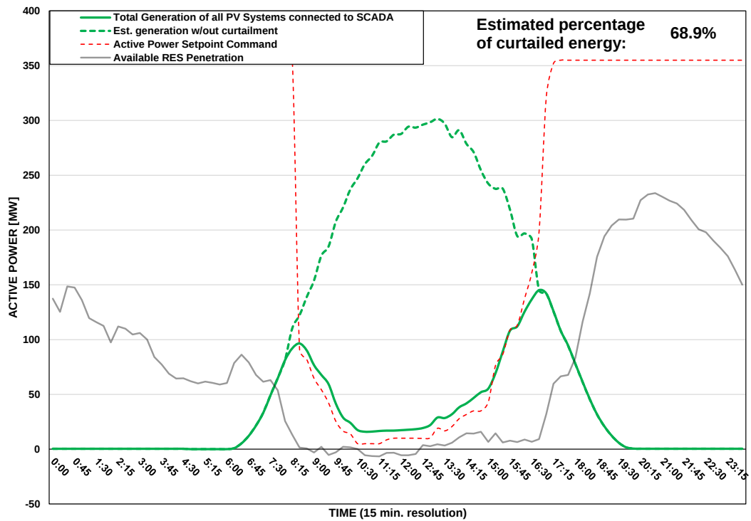
Scada PVs Generation on 03/08/2025 (curtailment time: 08:15 - 16:30)
