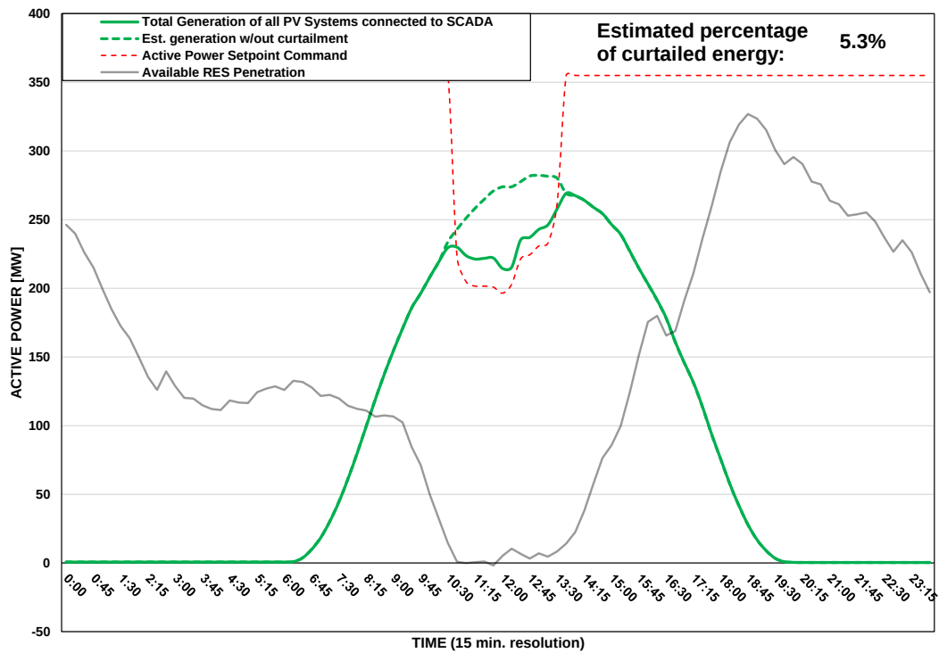
Scada PVs Generation on 11/08/2025 (curtailment time: 10:30 - 13:30)
