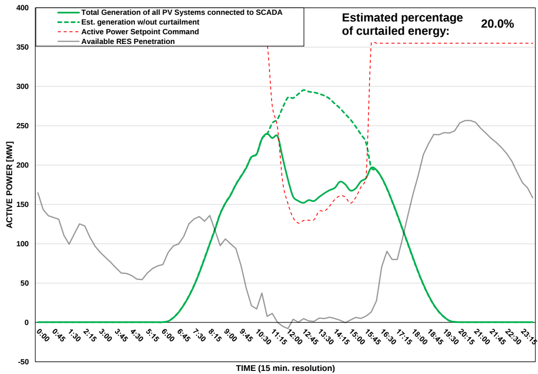
Scada PVs Generation on 30/07/2025 (curtailment time: 11:15 - 15:45)
