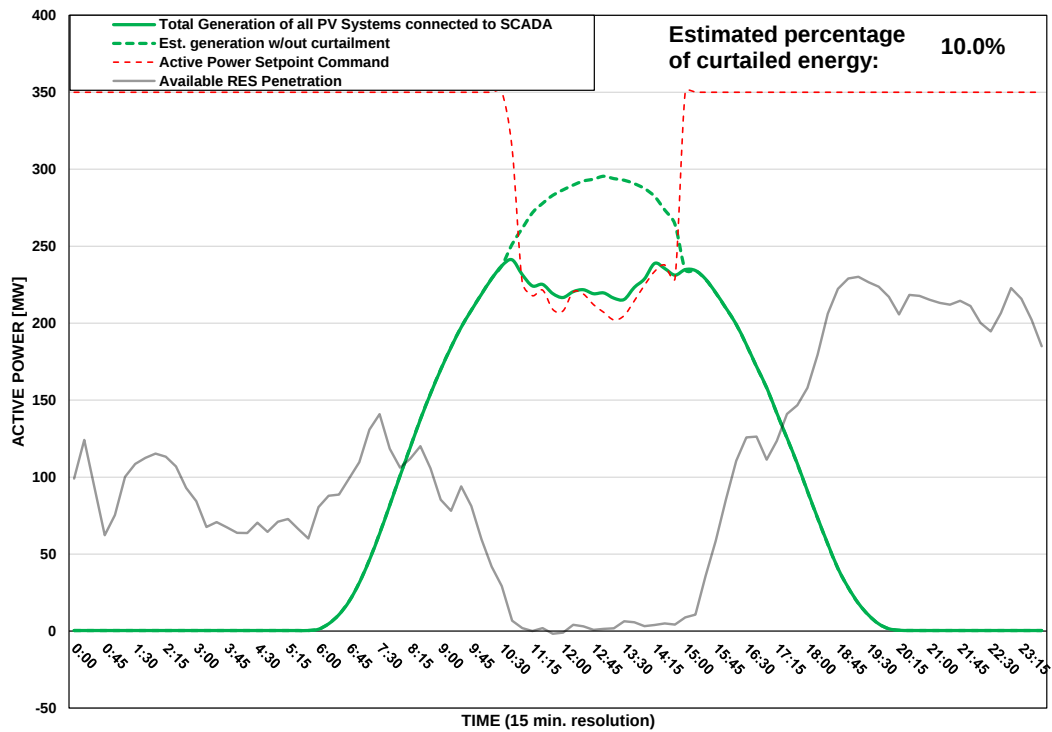
Scada PVs Generation on 08/07/2025 (curtailment time: 10:45 - 14:45)
