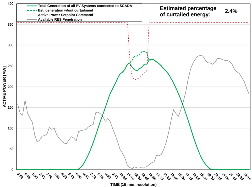
Scada PVs Generation on 29/07/2025 (curtailment time: 11:30 - 13:15)
