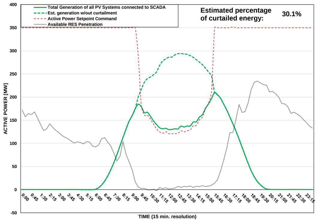
Scada PVs Generation on 12/07/2025 (curtailment time: 09:30 - 15:30)
