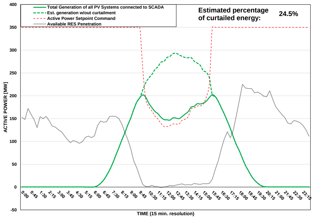
Scada PVs Generation on 18/07/2025 (curtailment time: 10:00 - 15:30)
