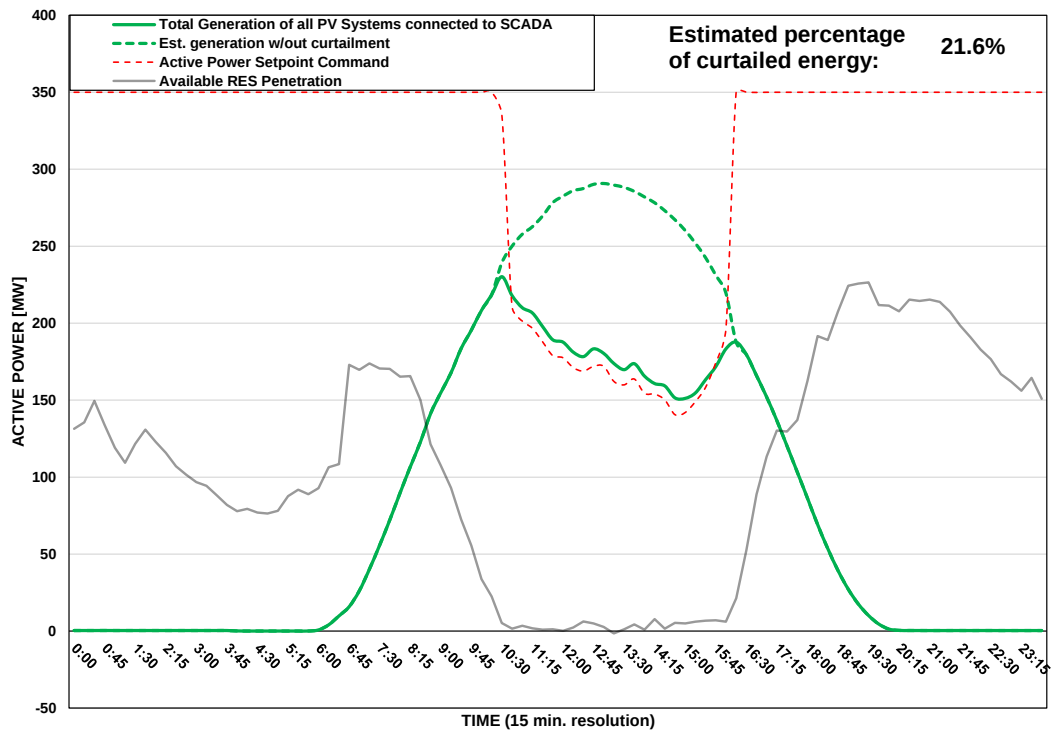
Scada PVs Generation on 14/07/2025 (curtailment time: 10:30 - 16:00)
