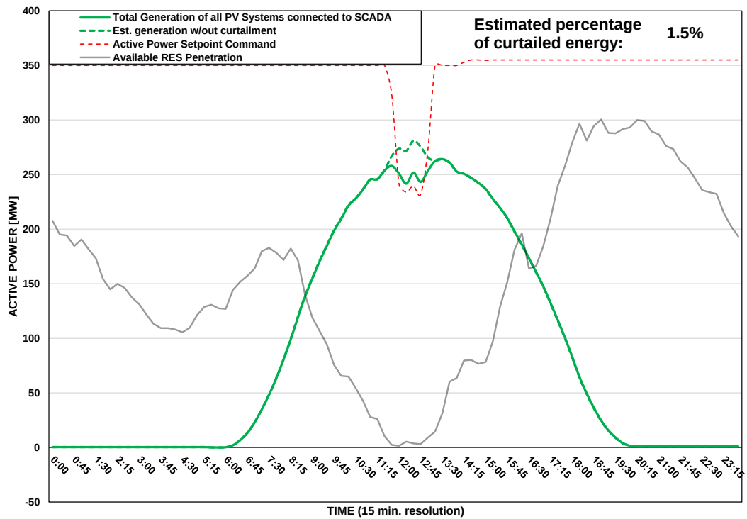
Scada PVs Generation on 21/07/2025 (curtailment time: 11:45 - 13:00)
