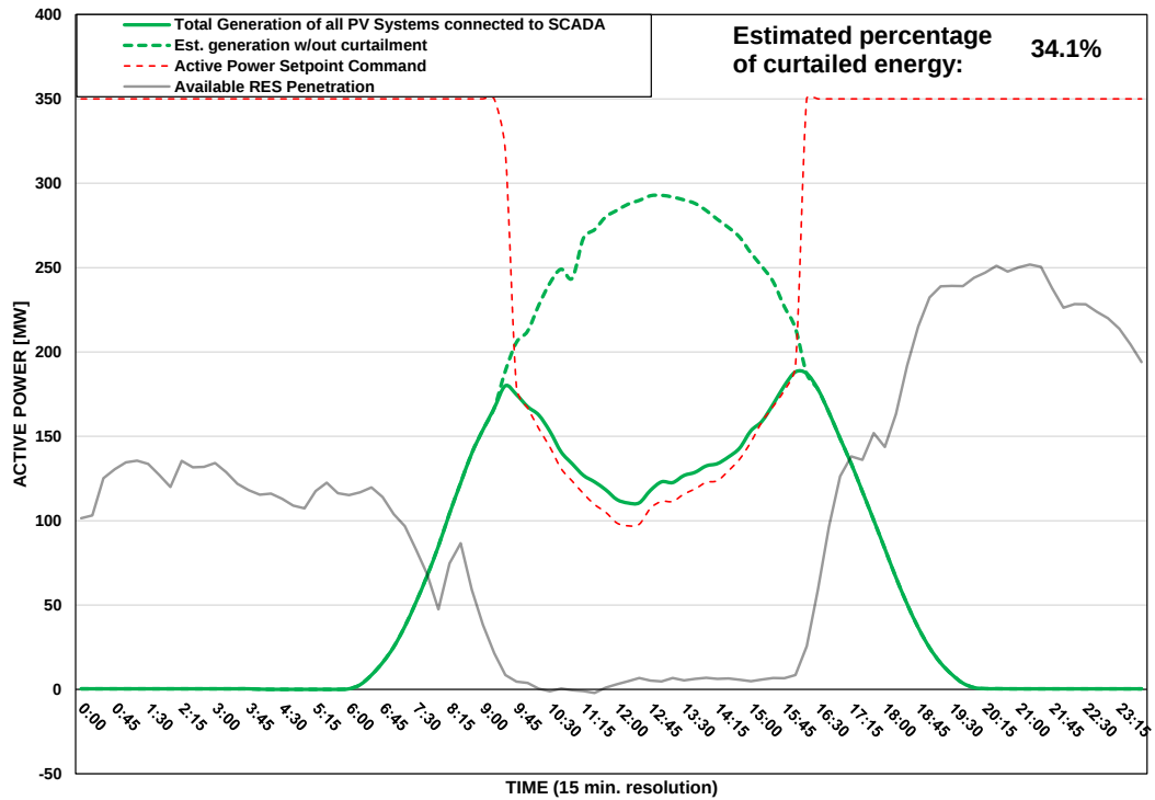
Scada PVs Generation on 19/07/2025 (curtailment time: 09:30 - 16:00)
