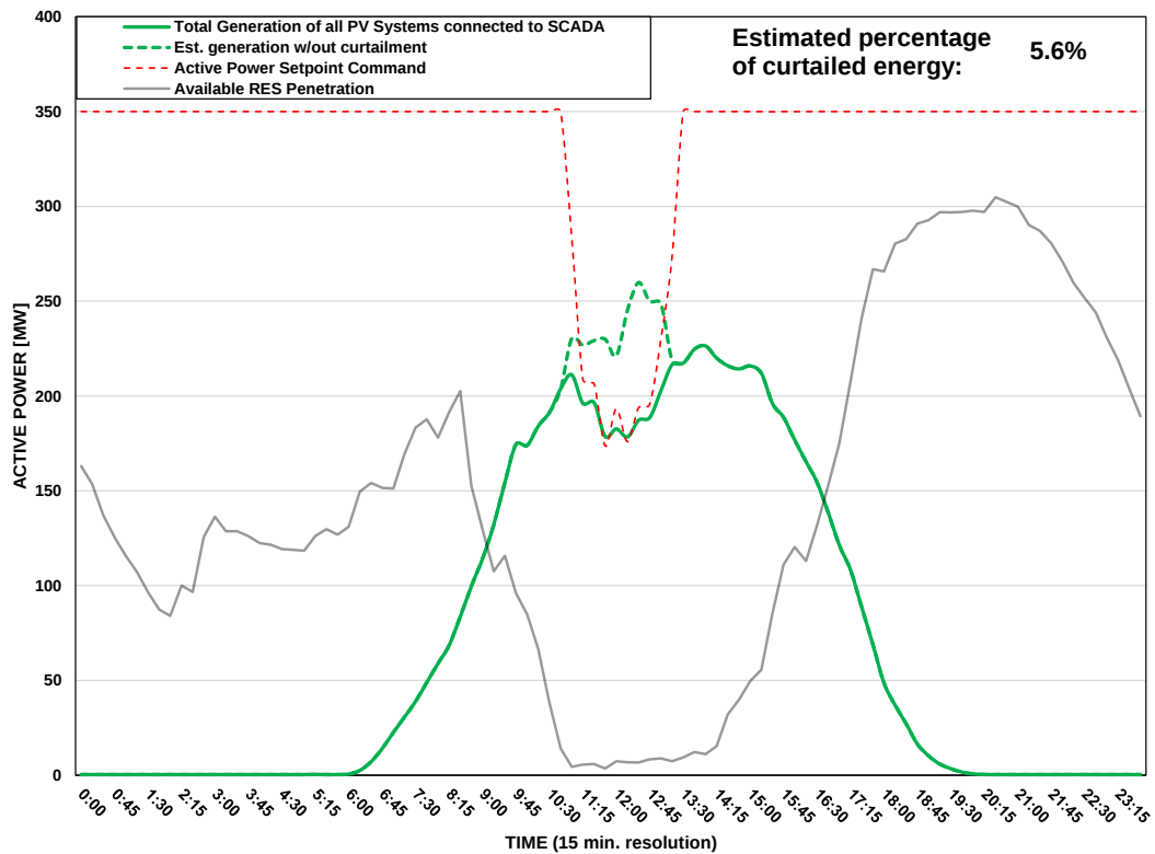
Scada PVs Generation on 16/07/2025 (curtailment time: 11:00 - 13:15)
