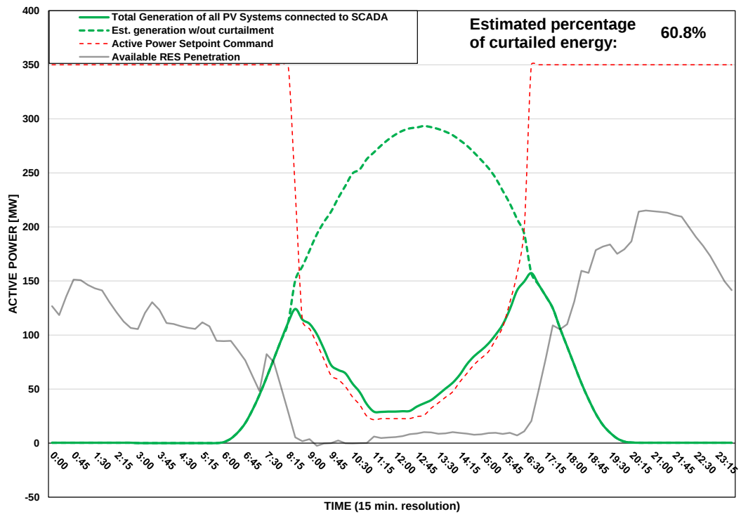
Scada PVs Generation on 13/07/2025 (curtailment time: 08:30 - 16:30)
