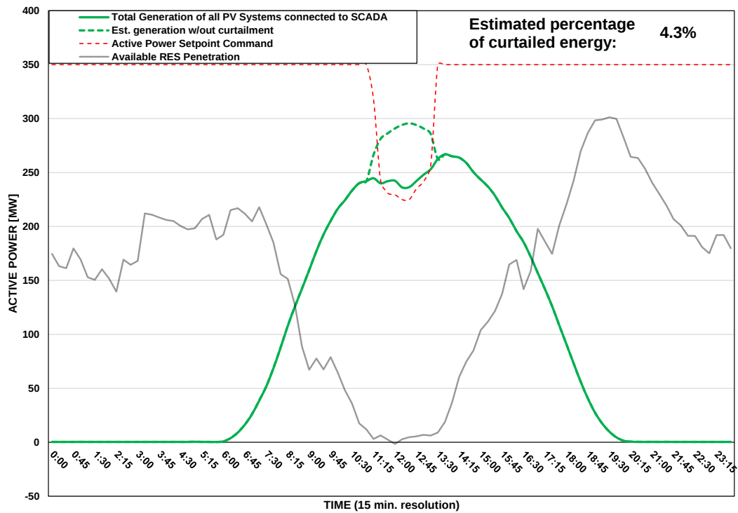
Scada PVs Generation on 11/07/2025 (curtailment time: 11:15 - 13:15)
