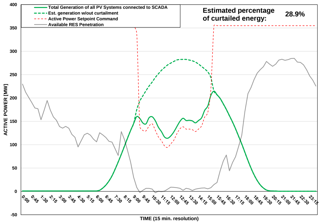
Scada PVs Generation on 27/07/2025 (curtailment time: 09:15 - 15:15)
