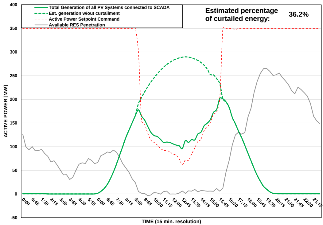
Scada PVs Generation on 02/07/2025 (curtailment time: 09:15 - 15:45)
