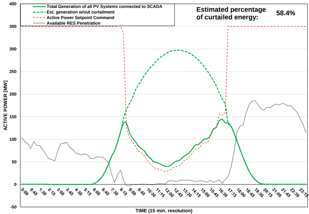
Scada PVs Generation on 06/07/2025 (curtailment time: 08:30 - 17:00)
