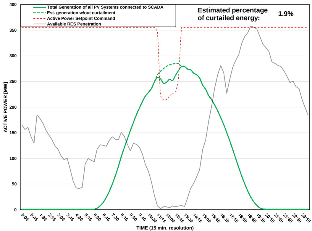
Scada PVs Generation on 23/07/2025 (curtailment time: 11:15 - 13:00)
