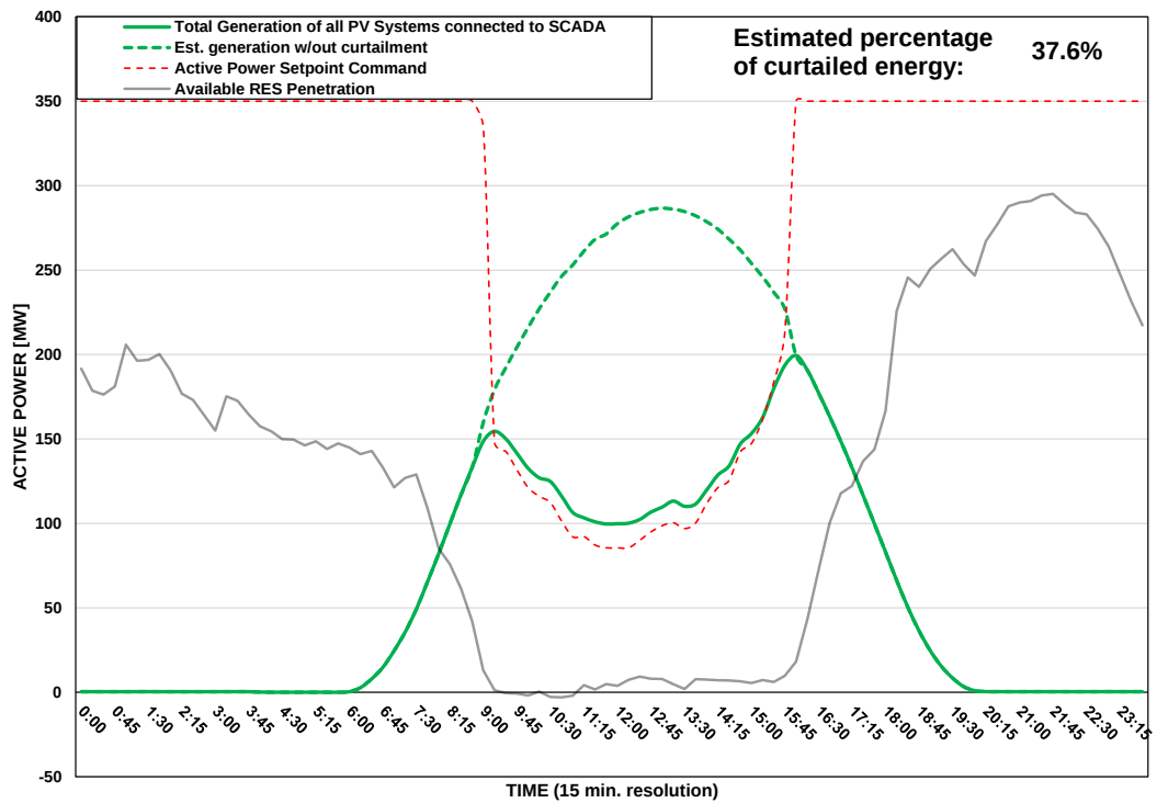
Scada PVs Generation on 20/07/2025 (curtailment time: 09:00 - 15:45)
