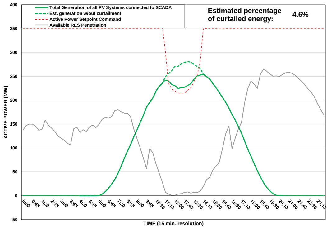
Scada PVs Generation on 15/07/2025 (curtailment time: 11:15 - 14:00)
