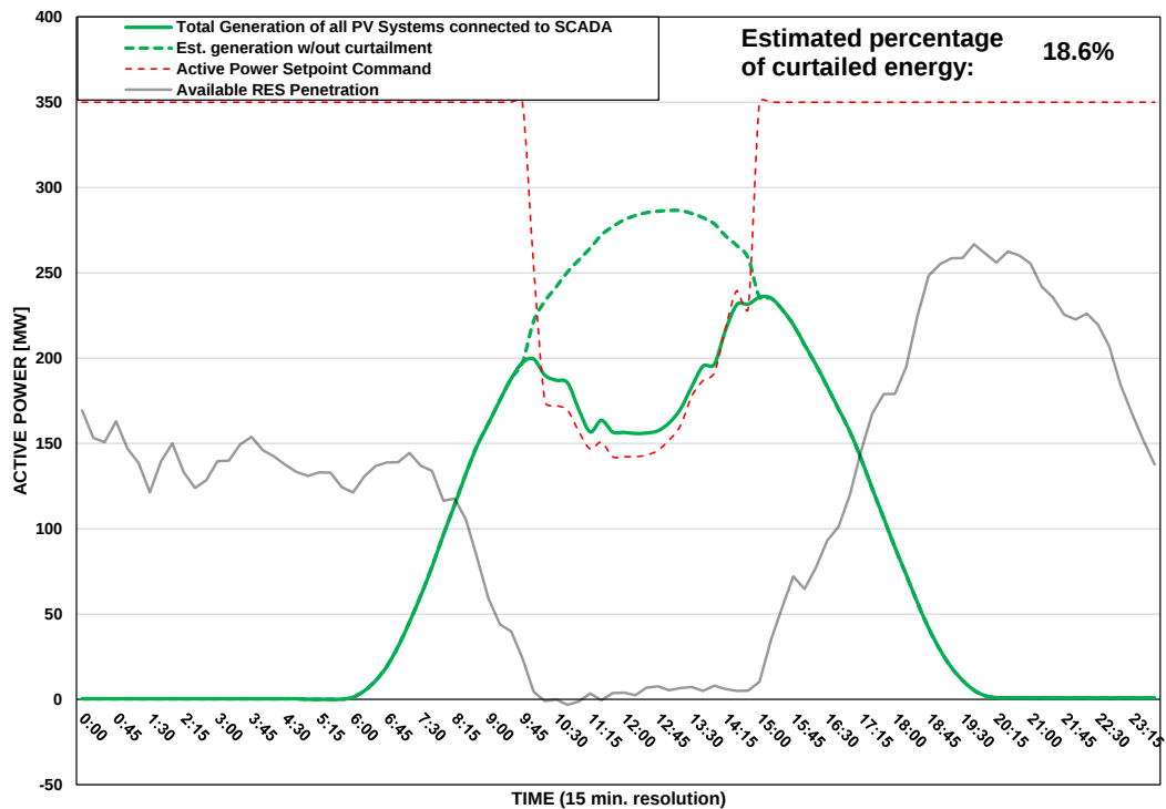
Scada PVs Generation on 09/07/2025 (curtailment time: 10:00 - 14:45)
