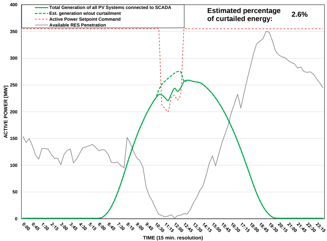
Scada PVs Generation on 26/07/2025 (curtailment time: 10:45 - 12:30)
