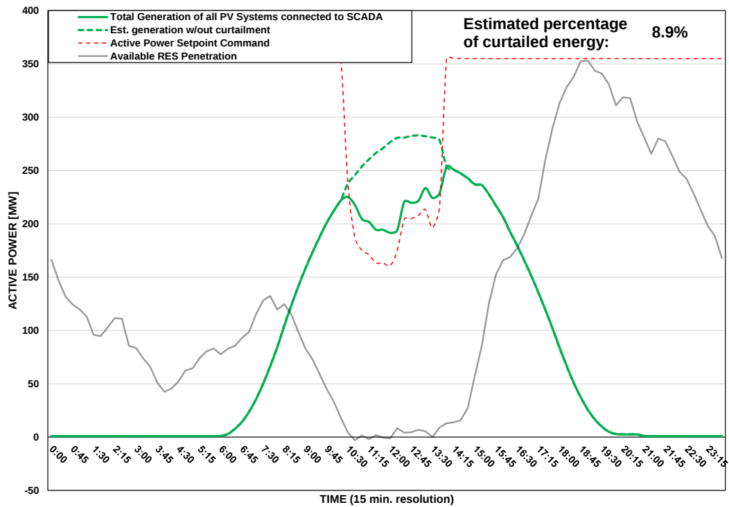
Scada PVs Generation on 24/07/2025 (curtailment time: 10:30 - 13:45)
