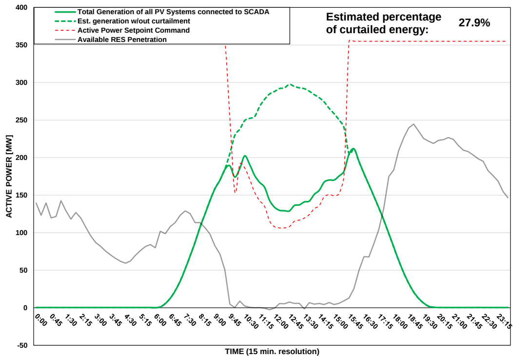
Scada PVs Generation on 31/07/2025 (curtailment time: 09:45 - 15:30)
