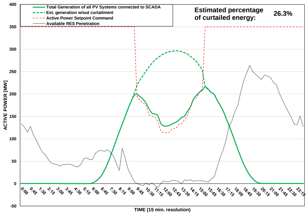
Scada PVs Generation on 03/07/2025 (curtailment time: 09:30 - 15:15)
