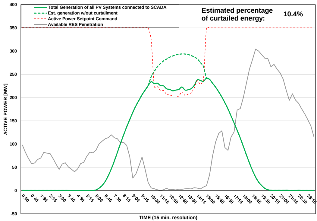
Scada PVs Generation on 07/07/2025 (curtailment time: 10:30 - 14:45)
