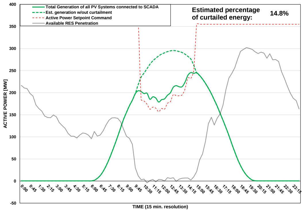
Scada PVs Generation on 28/07/2025 (curtailment time: 10:00 - 14:45)
