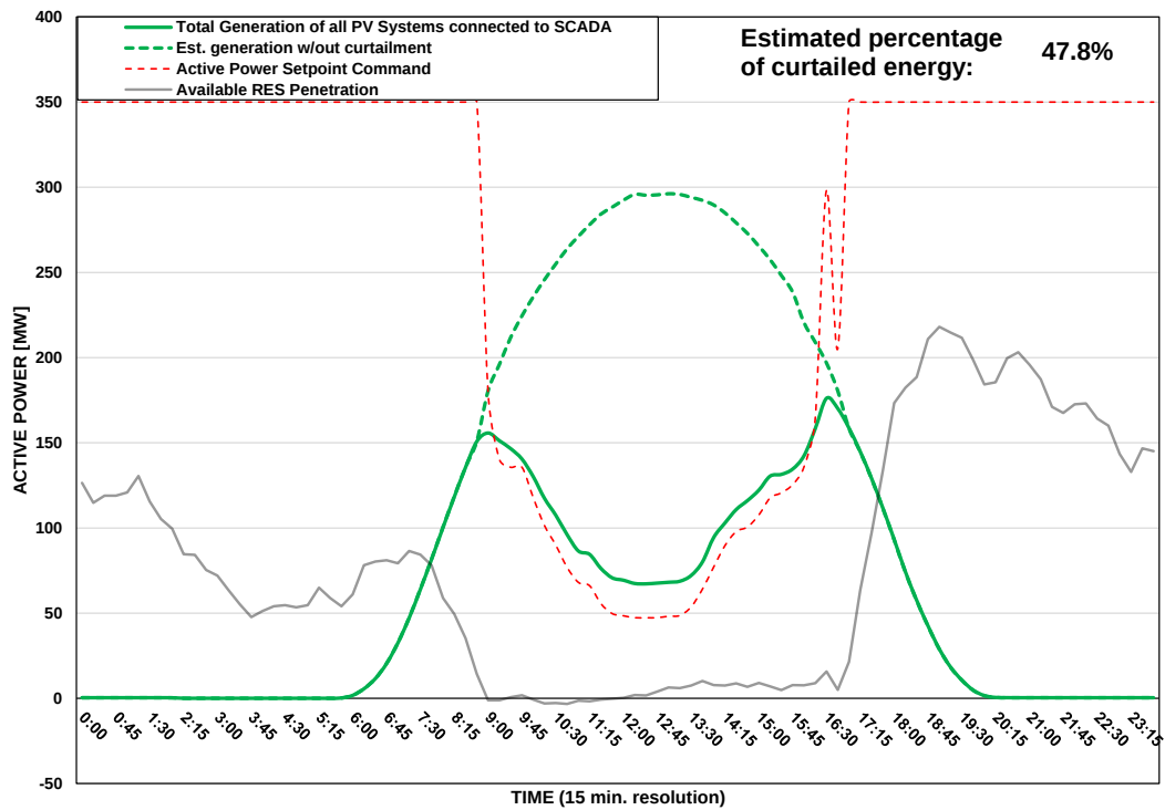
Scada PVs Generation on 01/07/2025 (curtailment time: 09:00 - 16:45)
