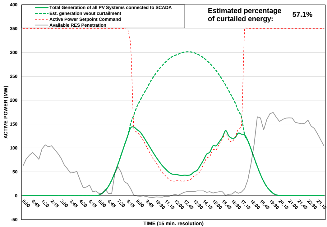
Scada PVs Generation on 05/07/2025 (curtailment time: 08:30 - 17:15)
