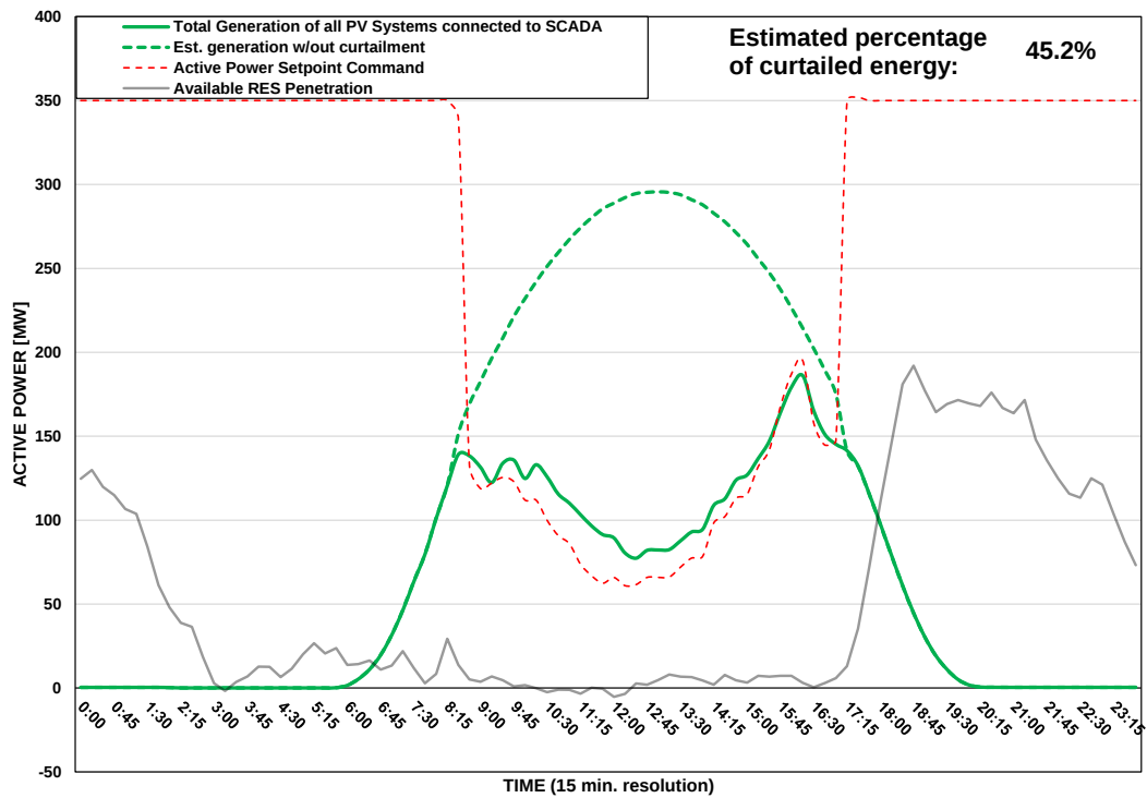
Scada PVs Generation on 04/07/2025 (curtailment time: 08:30 - 17:00)
